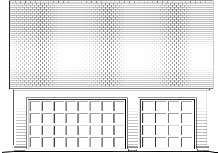
Front Elevation
